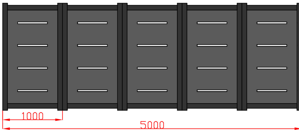
Assembly Diagram 1:2
